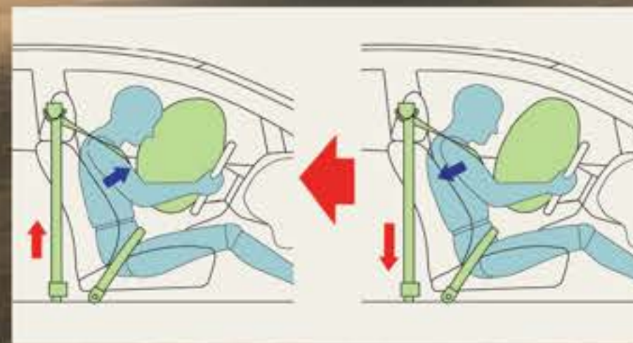
Front Seat Belts: 3-Point ELR with Pretensioner and Force Limiter
